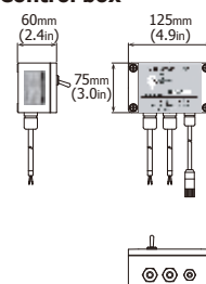
Control box
