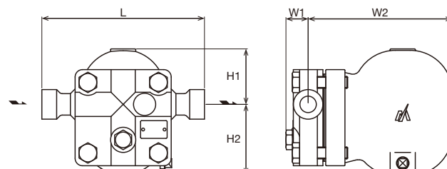
GTH12 Screwed GTH12-W Socket Weld
