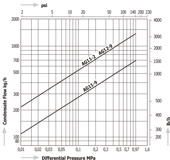
Capacity Chart AG11, AG12
