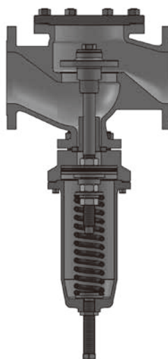
Size: DN 125 – 200
