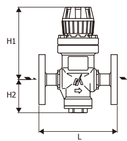
Dimensions REC1 - Flanged
