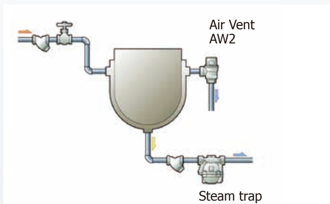
Open boiler
