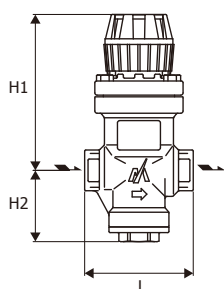
Dimensions REC1 - Screwed
