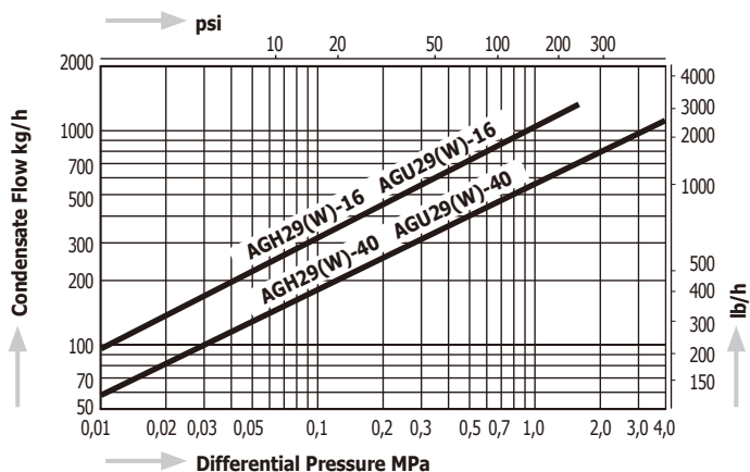
Capacity Chart AGH29, AGU29
