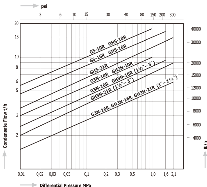
Capacity Chart
