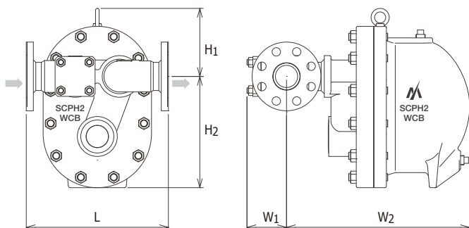
Dimensions GH60
