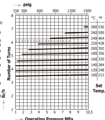
TBH71 - 105
