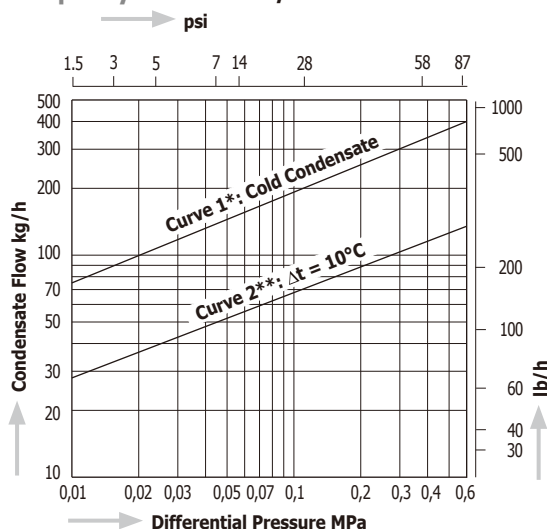
Capacity Chart TBU4/TBU4B-6
