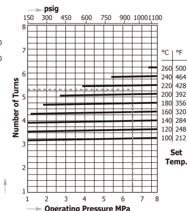
TBH71 - 80
