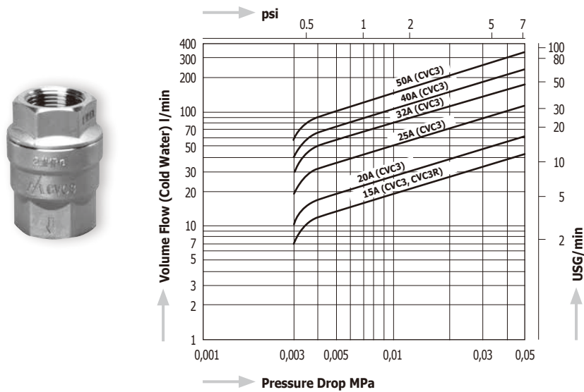
Pressure Drop Chart
