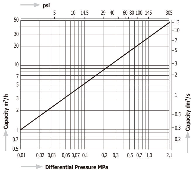
Capacity Chart AVG1V
