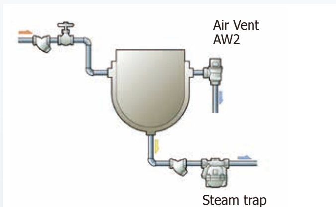
Open boiler
