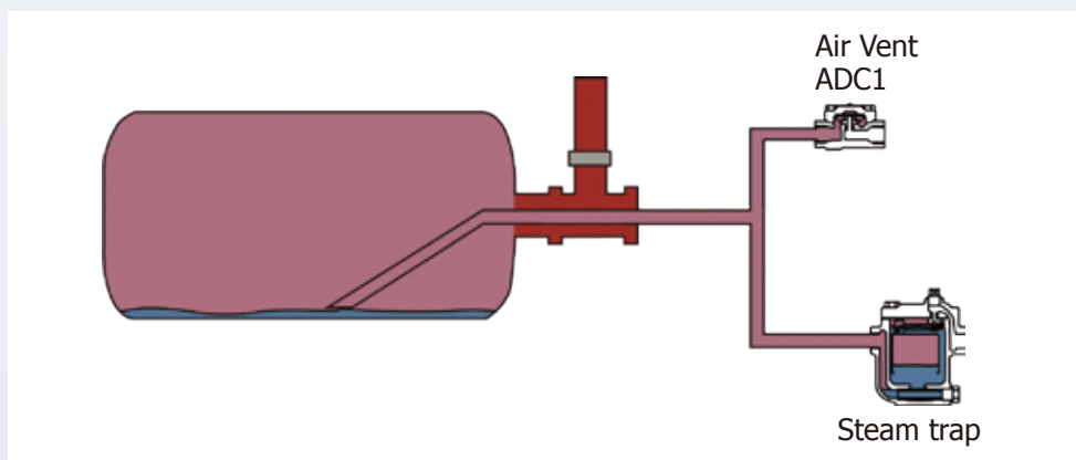
Drum dryer
