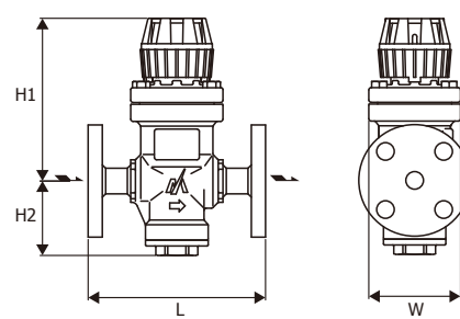
Dimensions REC1 - Flanged
