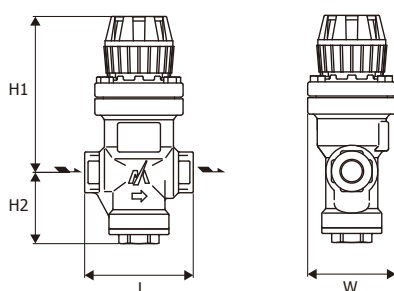
Dimensions REC1 - Screwed
